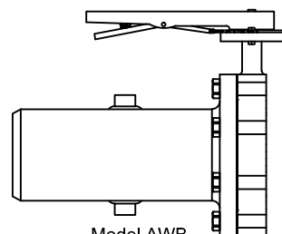
Model AWB Weld x Butterfly Valve
