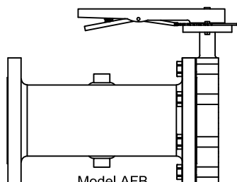
Model AFB Flange x Butterfly Valve
